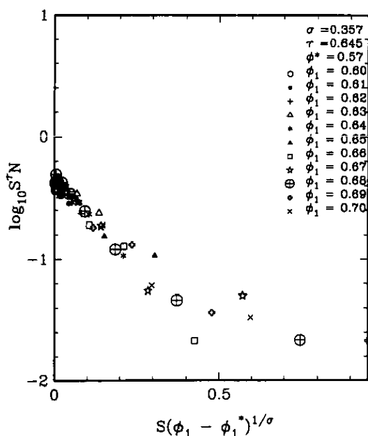
Figure 6. Scaling plot of the burst size in terms of cells S(b, c) . Here \log_{10} S(b, c)^{\tau(b,c)} N_{S(b,c)} is plotted as a function of [\phi_1 - \phi_1^*(b, c)]^{1/\sigma(b,c)} S(b, c) as in relation (5). The best collapse of the data is for \sigma(b, c) = 0.36 , \tau(b, c) = 0.65 and \phi_1^*(b, c) = 0.57 .
