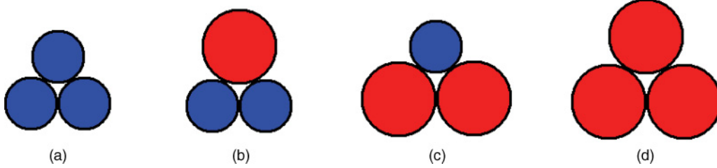
FIG. 13. (Color online) The four distinct three-particle loops in a binary circular disk packing.
