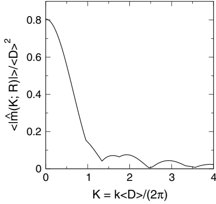
FIG. 5. The average magnitude \langle |\hat{m}(k; R)| \rangle_R of the spatial contribution to the spectral density.
