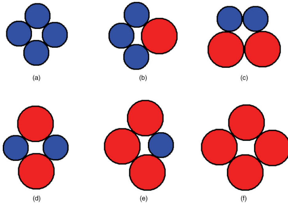
FIG. 14. (Color online) The six distinct families of four-particle loops in a binary circular disk packing.
