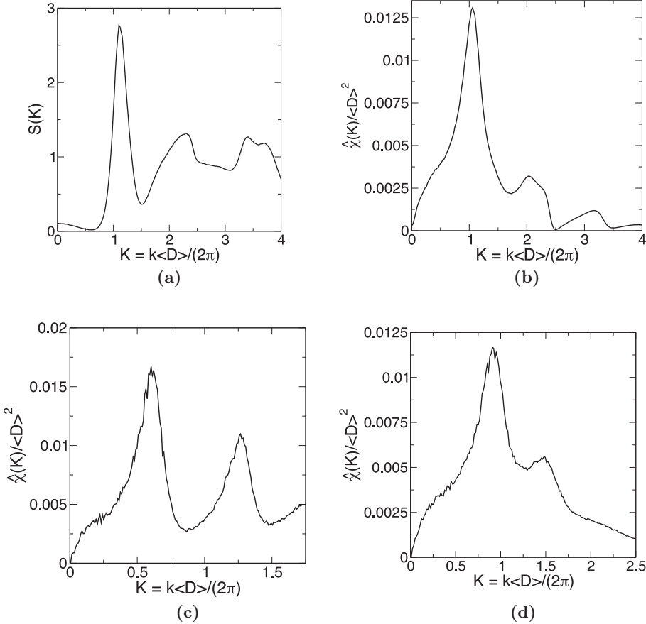
FIG. 2. (a) Structure factor S(k) for a binary packing of disks near the MRJ state. (b) The corresponding spectral density \hat{\chi}(k) . Note that infinite-wavelength local density fluctuations are not suppressed, unlike local-volume-fraction fluctuations on the equivalent length scale. (c) Spectral density for particle concentrations \gamma_{\text{small}} = 2/3 and \gamma_{\text{large}} = 1/3 with size ratio \beta = 2.5 . Hyperuniformity of the packing is unaffected by changes in these parameters as expected by the Torquato-Stillinger conjecture. (d) Spectral density for a polydisperse MRJ packing of disks with a uniform distribution of radii in the interval [R_{\text{min}}, R_{\text{max}}] .
