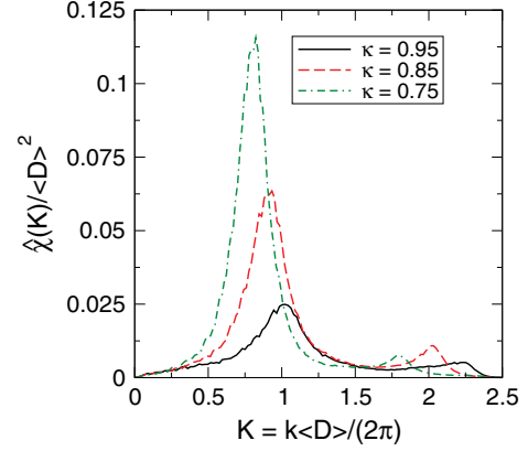
FIG. 9. (Color online) Spectral densities upon shrinking the particles in the binary MRJ packings at fixed size ratio \beta = R_{\text{large}}/R_{\text{small}} . The parameter \kappa = R_{\text{shrink}}/R_{\text{MRJ}} is the scaling factor.
