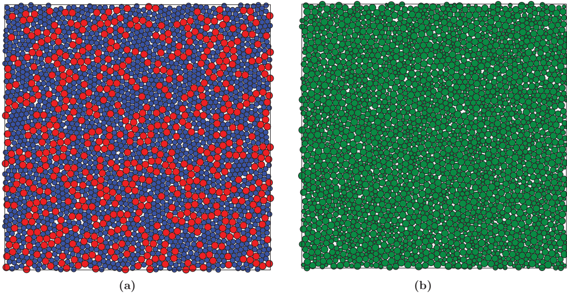
FIG. 1. (Color online) (a) A binary packing of hard disks near the MRJ state. (b) A polydisperse packing of hard disks near the MRJ state.
