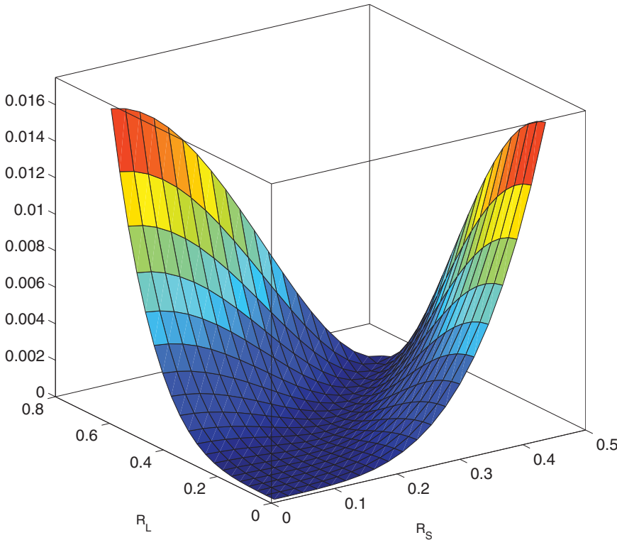
FIG. 10. (Color online) The quadratic form (35), equal to the small-wave-number limit of the spectral density \chi(0) , as a function of the radii of the particles in the packing. A uniform decrease in the particle radii defines a basin of hyperuniform systems.
