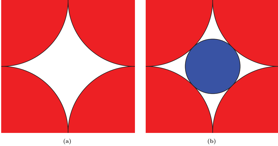
FIG. 8. (Color online) (a) Unit cell for the square lattice at close packing. (b) Unit cell for a close-packed binary variant of the square lattice.
