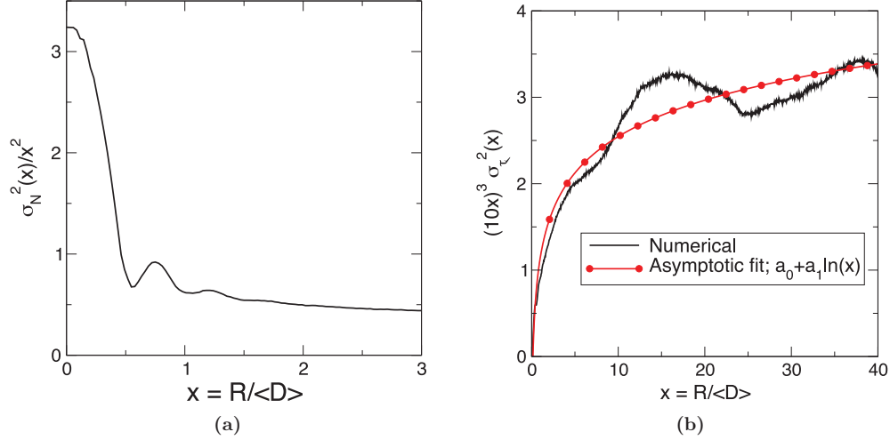
FIG. 3. (Color online) (a) Asymptotic fluctuations in the local number density for the MRJ binary disk packing. (b) Asymptotic fluctuations in the local volume fraction for the binary MRJ packing, demonstrating that the system is indeed hyperuniform.
