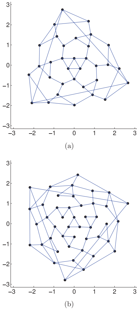
FIG. 13. (Color online) As in Fig. 8, except, here, we show the last shells of the N = 45 and N = 57 DLP optimal packings, both of which belong to point group C_3 . For both shells, the zenith direction is chosen along one of the C_3 axes shared by all shells in the packing. (a) Thirty-three spheres, R = R_{\min}(45) = 1.749\,669\dots , point group C_3 . (b) Forty-five spheres, R = R_{\min}(57) = 1.877\,196\dots , point group C_3 .
