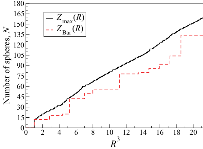
FIG. 1. (Color online) Z_{\max}(R) vs R^3 , as determined by optimal and putatively optimal solutions to the DLP problem for N = 1 to N = 161 , and Z_{\text{Bar}}(R) . The radius R of the sphere enclosing the centers of the N identical (smaller) spheres and the same-size fixed sphere is measured in units of the diameter of the enclosed spheres.
