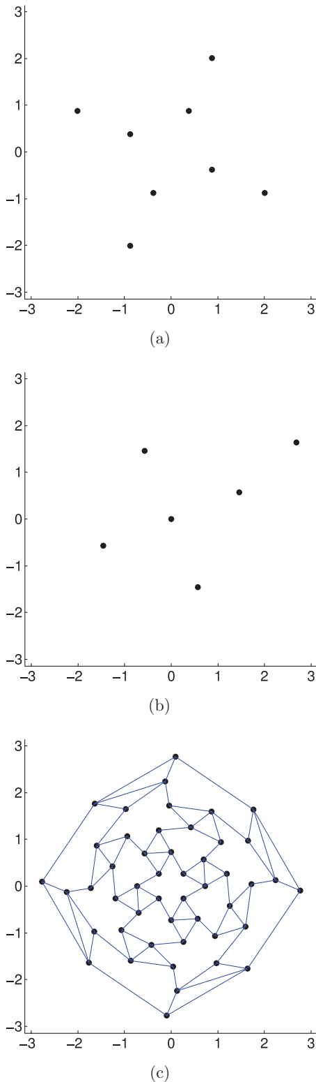
FIG. 10. (Color online) As in Fig. 8, except, here, we show the three shells of the N = 62 DLP optimal packing, which belongs to point group O . The zenith direction is chosen along one of the C_4 axes shared by all three shells. (a) Eight spheres, R = 1.087541\dots , point group O_h . (b) Six spheres, R = 1.087785\dots , point group O_h . In this projection, as the sphere center furthest from the origin is at distance \pi (corresponding in \mathbb{R}^3 to an angle of inclination equal to \pi ), its azimuthal angle is chosen at random. (c) R = R_{\min}(62) = 1.927715\dots , point group O .
