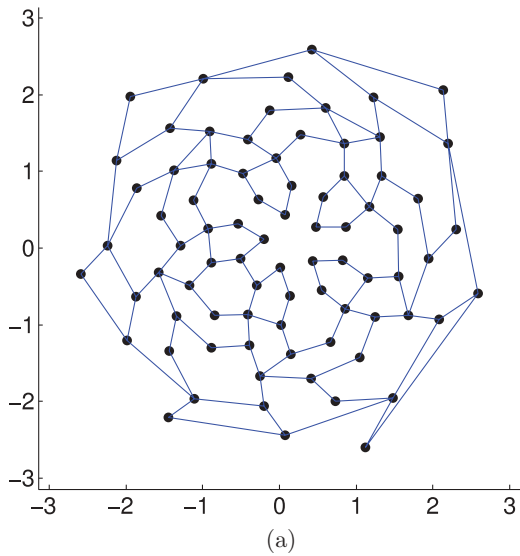
FIG. 17. (Color online) As in Fig. 8, except, here, we show the last shell of the roughly icosahedrally symmetric N = 134 DLP optimal packing, including 80 spheres with centers at distance R_{\min}(134) = 2.585\ 815\dots . The centers of 60 of the spheres roughly form the vertices of a truncated icosahedron, while the remaining 20 spheres are centered in the truncated icosahedron’s hexagonal faces. The zenith direction is chosen along one of the rough C_5 axes.
