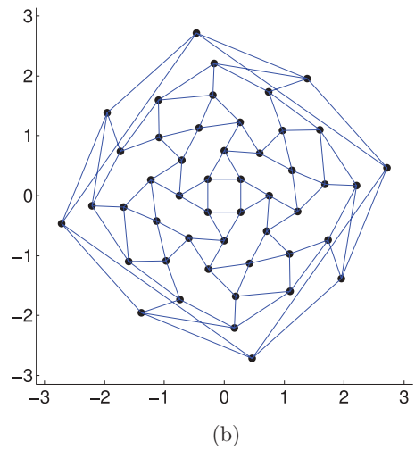
FIG. 9. (Color online) As in Fig. 8, except, here, we show the two shells of the N = 60 DLP optimal packing, which belongs to point group O . The zenith direction is chosen along one of the C_4 axes shared by both shells. (a) Twelve spheres, R = 1 , point group O_h . (b) Forty-eight spheres, R = R_{\min}(60) = 1.891\,101\dots , point group O .
