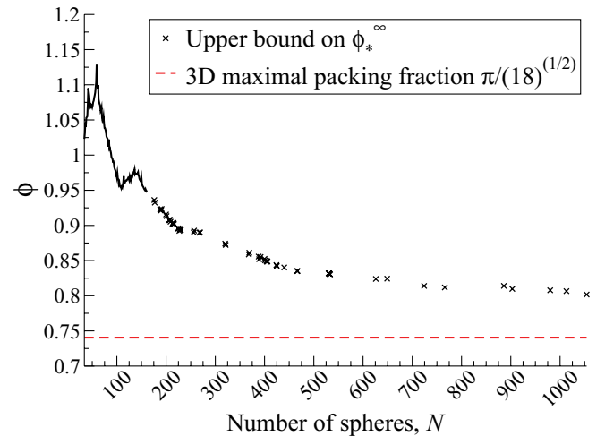
FIG. 3. (Color online) An upper bound on \phi_*^\infty in \mathbb{R}^3 as calculated from the putative R_{\min}(N) for N = 34 to N = 161 and for selected values of N \geq 176 , vs the (known) maximal packing fraction \phi_*^\infty of an infinite packing of identical nonoverlapping spheres in \mathbb{R}^3 , \phi_*^\infty = \pi/\sqrt{18} \approx 0.7405 .
