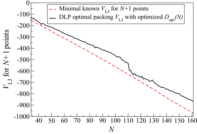
FIG. 7. (Color online) Plot of the minimum known [33] V_{LJ}(\mathbf{r}^{N+1}) , Eq. (10), for N + 1 points vs the V_{LJ} of DLP optimal packings with spheres of optimized diameter D_{\text{opt}}(N) for N = 34 to N = 161 .
