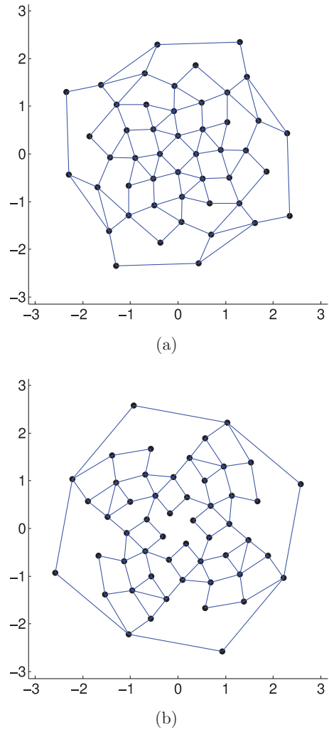
FIG. 14. (Color online) As in Fig. 8, except, here, we show the jammed spheres in the last shells of the N = 61 and N = 74 DLP optimal packings, both of which belong to point group C_4 . For both shells, the zenith direction is chosen along one of the C_4 axes. (a) Forty-eight spheres, R = R_{\min}(61) = 1.919\,926\dots , point group C_4 . (b) Fifty-two jammed spheres (of 56 total in the shell), R = R_{\min}(74) = 2.077\,792\dots , point group C_4 .
