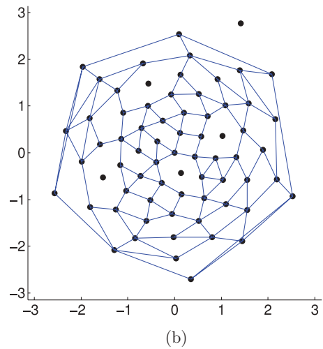
FIG. 18. (Color online) As in Fig. 8, except, here, we show the first and only shells for the N = 77 and N = 93 “maracas” packings, including rattlers. The zenith direction in each case is chosen somewhat arbitrarily to run through the center of one of the surrounding spheres. (a) Fifty-nine spheres, one rattler, R_{\min}(77) = 2.111\ 526\dots , point group C_1 . (b) Sixty-nine spheres, five rattlers, R = R_{\min}(93) = 2.280\ 243\dots , point group C_1 .
