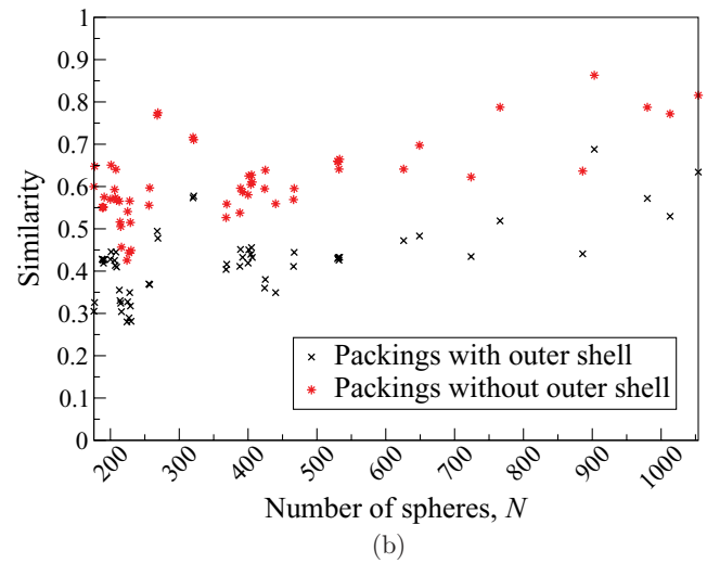
FIG. 5. (Color online) Similarity metric from Eq. (9). An X represents the maximal similarity calculated for the comparisons of reference sets \mathbb{B}_N to a DLP optimal packing for N spheres. An * represents the maximal similarity for the comparisons of reference sets \mathbb{B}_M to a DLP optimal packing for N spheres with the N - M spheres with centers at distance R_{\min}(N) removed.
