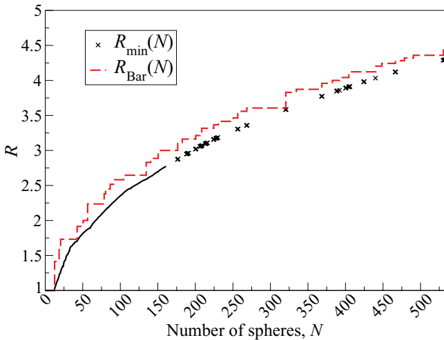
FIG. 2. (Color online) A plot of R_{\min}(N) vs N for N = 1 to N = 161 and for selected values of N \geq 176 , and R_{\text{Bar}}(N) vs N for N = 1 to N = 533 .
