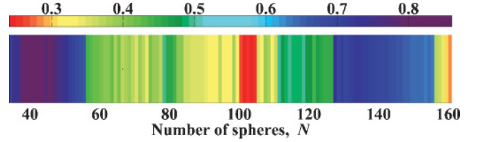
FIG. 6. (Color online) Similarity metric from Eq. (9), color coded as indicated in the key above the diagram, with violet-blue (darker shading) representing the highest values of \mathcal{S} and red-orange (lighter shading) representing the lowest. The value of \mathcal{S} displayed is calculated as the maximum for DLP optimal packings for a given N compared to the reference sets included in \mathbb{B}_N . Due to the similarity between subsets of fcc packings and certain packings with icosahedral symmetry, the ranges of N with highest \mathcal{S} , 34 \leq N \leq 55 and 127 \leq N \leq 155 , are radially and angularly distributed most similarly to a specific dense packing of spheres with perfect icosahedral symmetry.
