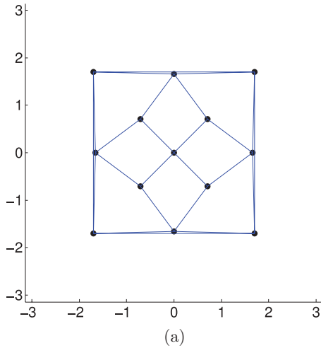
FIG. 8. (Color online) This plot is a projection from the surface of a sphere of radius R_{\min}(13) = 1.045\,572\dots of 13 points (sphere centers) in \mathbb{R}^3 to the interval [-\pi, \pi] \times [-\pi, \pi] in \mathbb{R}^2 . As the projection to \mathbb{R}^2 is most clearly defined in terms of polar coordinates and does not preserve distances from \mathbb{R}^3 , we do not provide labels for our axes. This DLP optimal packing contains only a single shell, the sphere centers of which belong to point group C_4 . In the projection, the angle of inclination of a point in \mathbb{R}^3 , represented in spherical coordinates, becomes the distance from the origin (radius) in \mathbb{R}^2 , while the azimuthal angle remains unchanged. Contacting spheres, i.e., spheres with centers (points) in \mathbb{R}^3 separated by unit distance where all spheres are of unit diameter, are connected by straight lines in the plot in \mathbb{R}^2 . The zenith direction from which each point's (sphere center's) angle of inclination is measured is chosen to coincide with the packing's C_4 axis; in this way, the projection to the plane preserves the rotational symmetry of the packing in \mathbb{R}^3 about the C_4 axis.
