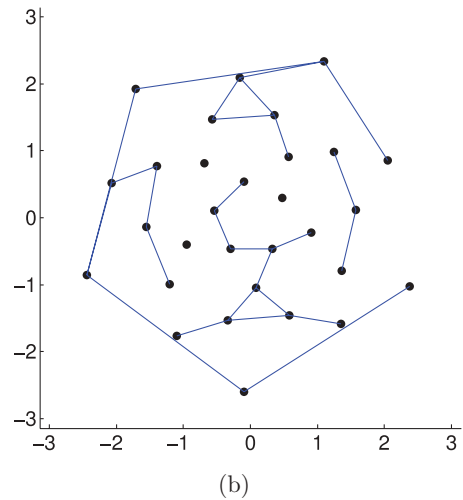
FIG. 16. (Color online) As in Fig. 8, except, here, we show the two shells of the N = 42 DLP optimal packing; the 12 sphere centers of the first shell roughly form the vertices of an icosahedron, and the 30 sphere centers (including 3 rattlers) of the second shell roughly form the vertices of an icosidodecahedron. The zenith direction in both cases is chosen along one of the rough C_5 axes. (a) Twelve spheres, R = 1 , point group I_h (to 0.012 sphere diameters). (b) Thirty spheres, R_{\min}(42) = 1.699423\dots , point group I_h (to 0.195 sphere diameters).
