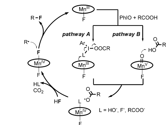
Figure 1. Mechanistic probes of the fluorine-transfer step.
